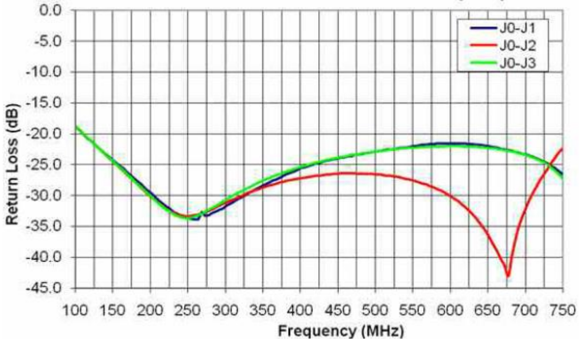
3100-150 Return Loss vs. Frequency
