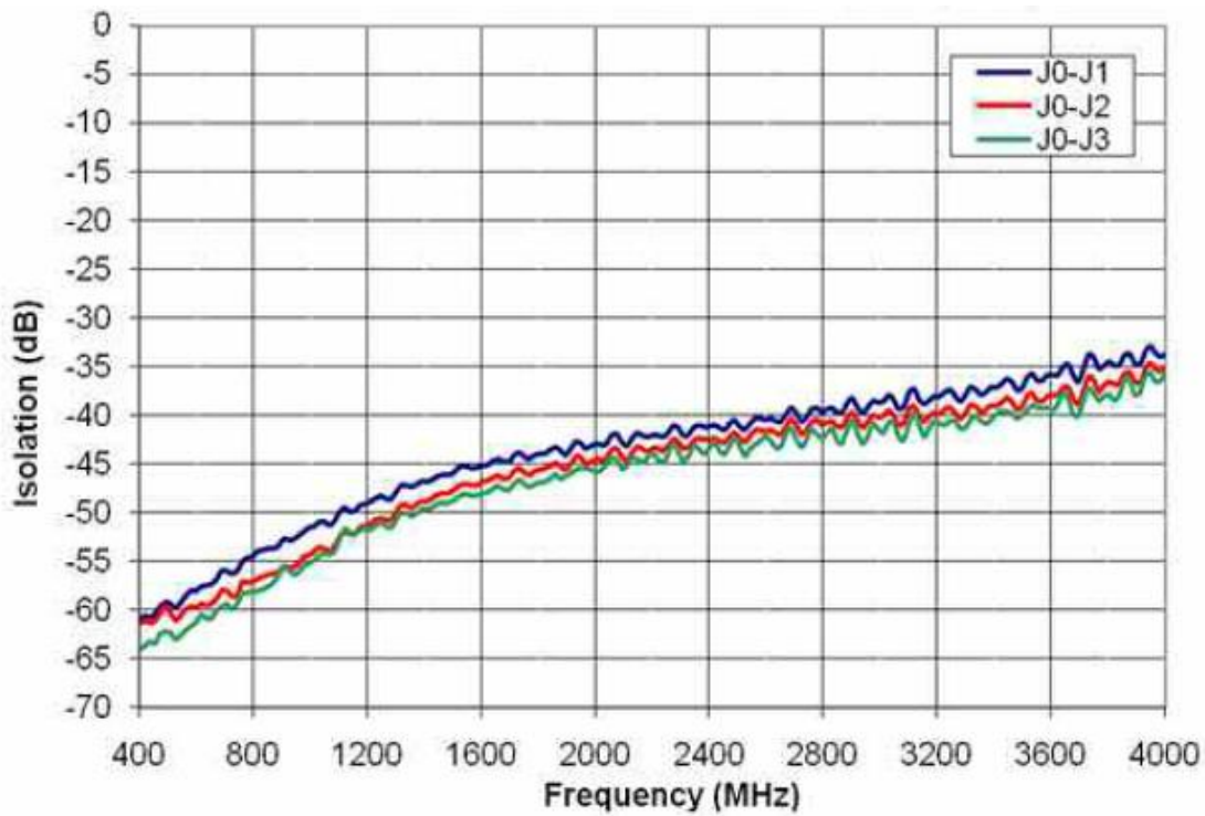
MSW3T-3101-150 Isolation vs. Frequency
