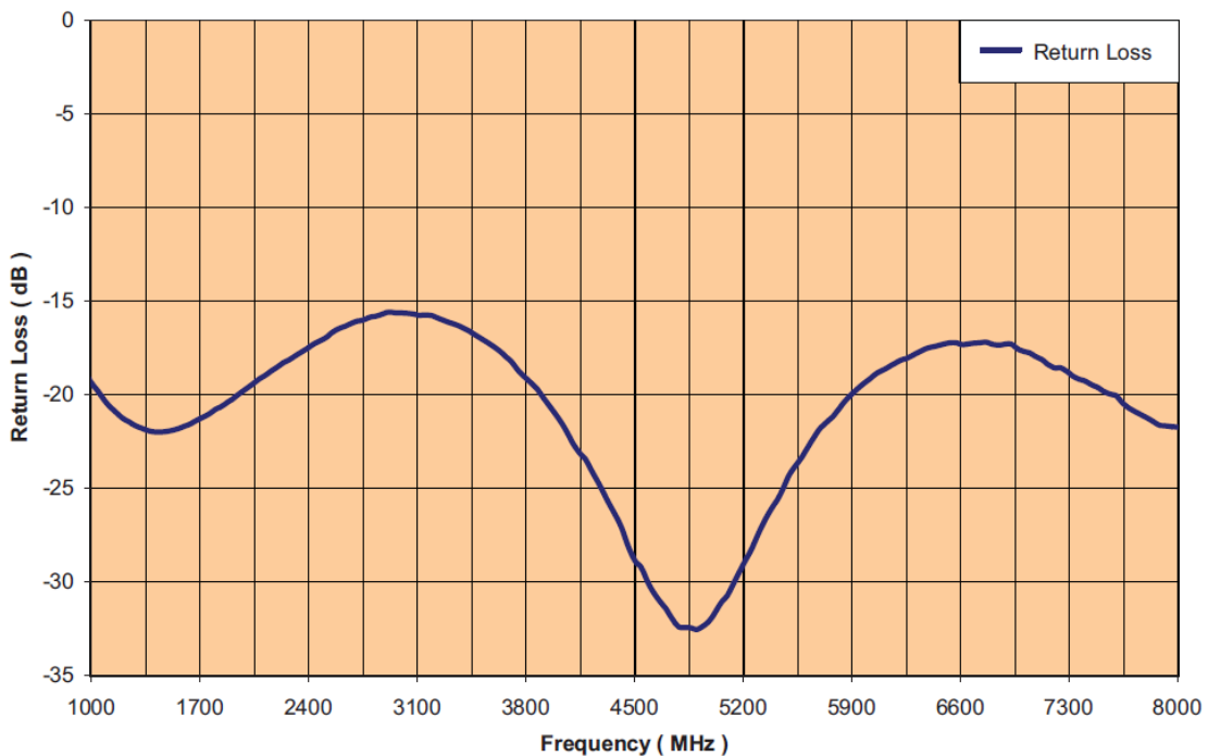
RFLM-202802QC-290 Return Loss vs Frequency
