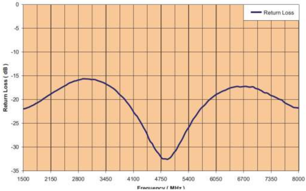
RFLM-202802LC-299 Return Loss vs Frequency
